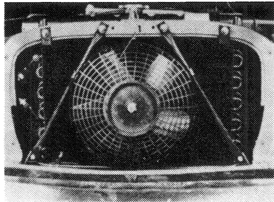
Fig. 3-7 1 — Auxiliary fan
